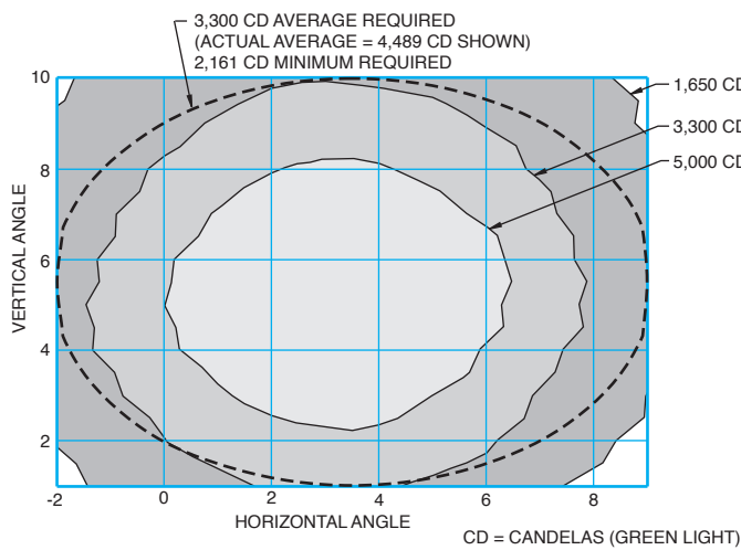
L-850D Inset Runway Threshold/End Light – Green
